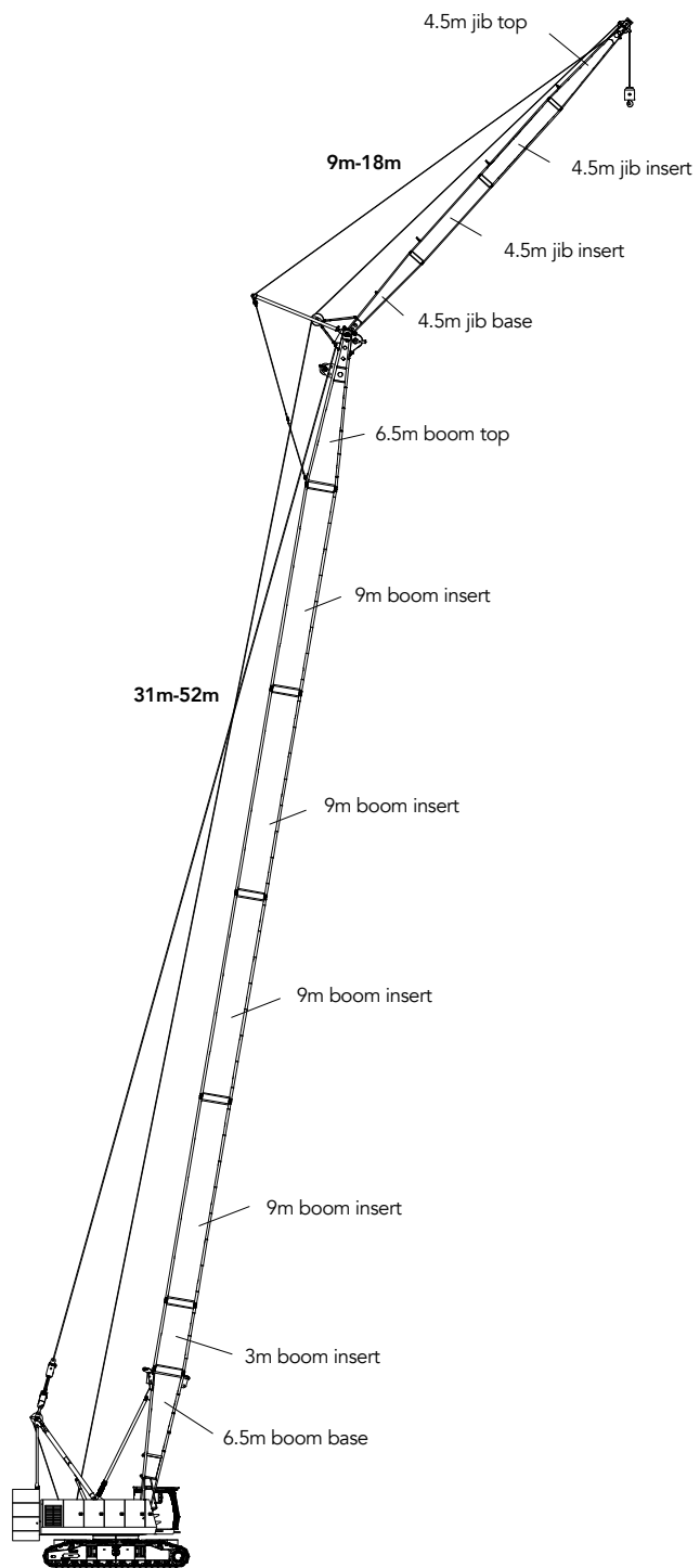
FJ Configuration
