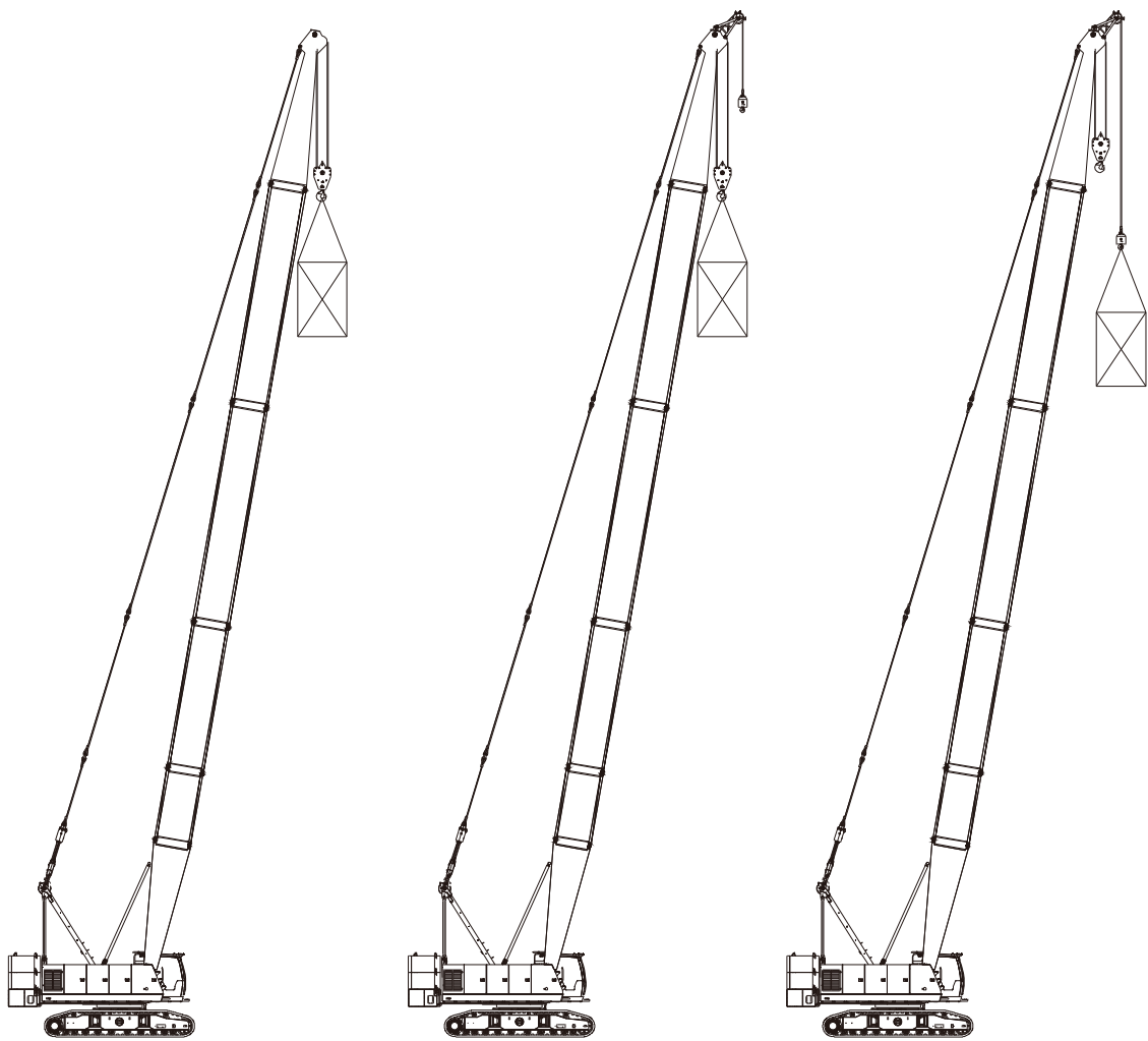
H Configuration
