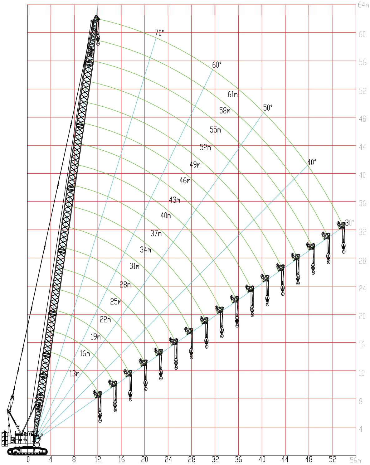
Crane working range: main boom working condition
